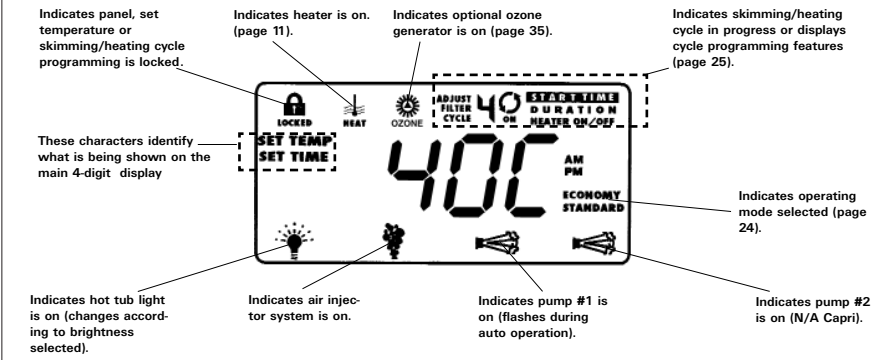
Figure-E, LCD Display
